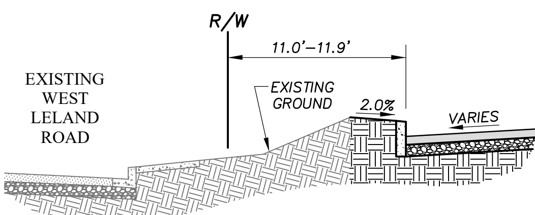
SECTION D-D NOT TO SCALE
