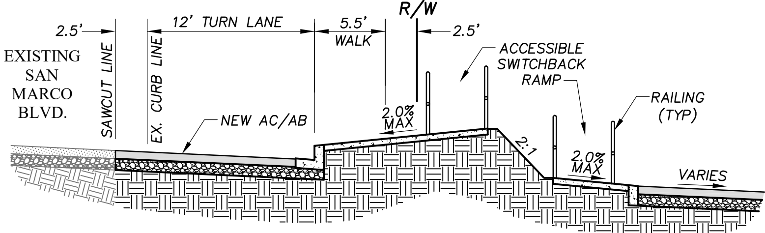
SECTION I-I NOT TO SCALE
