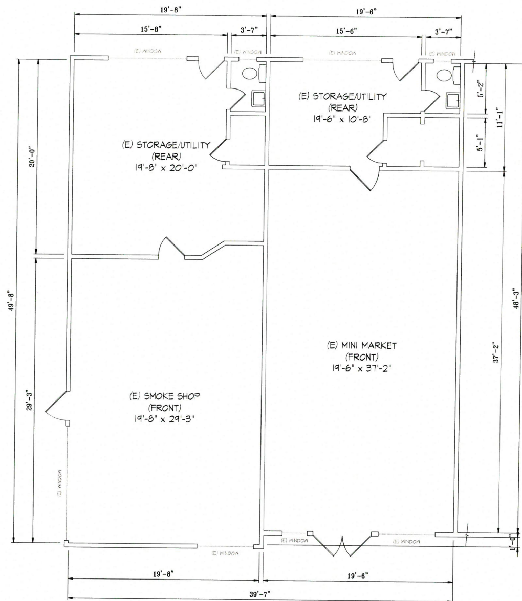
EXISTING FLOOR PLAN (FRONT SPACE SQFT: SMOKE SHOP = 610 SQFT / MINI MARKET = 756 SQFT) SCALE: 1/4" = 1'-0"
