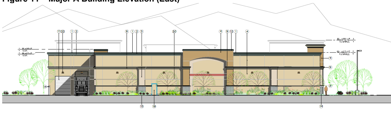
Figure 11 – Major A Building Elevation (East)
