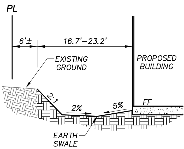
SECTION H-H NOT TO SCALE
