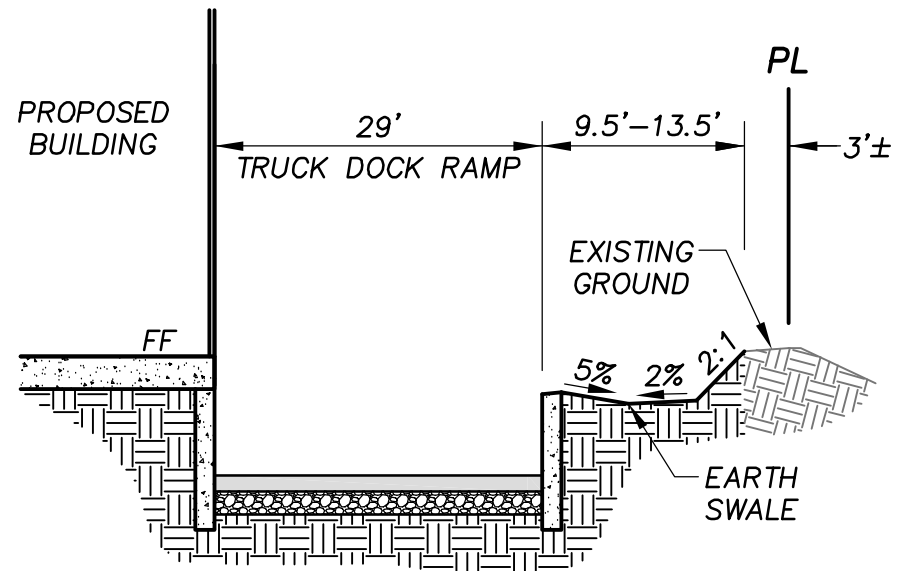
SECTION F-F NOT TO SCALE
