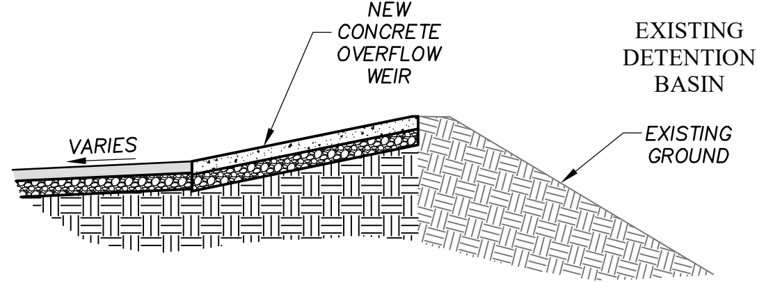
SECTION G-G NOT TO SCALE
